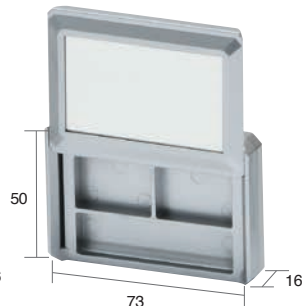
pan size : 27 x 18 C-0372A
